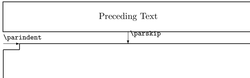
Figure 7: Paragraph parameters
